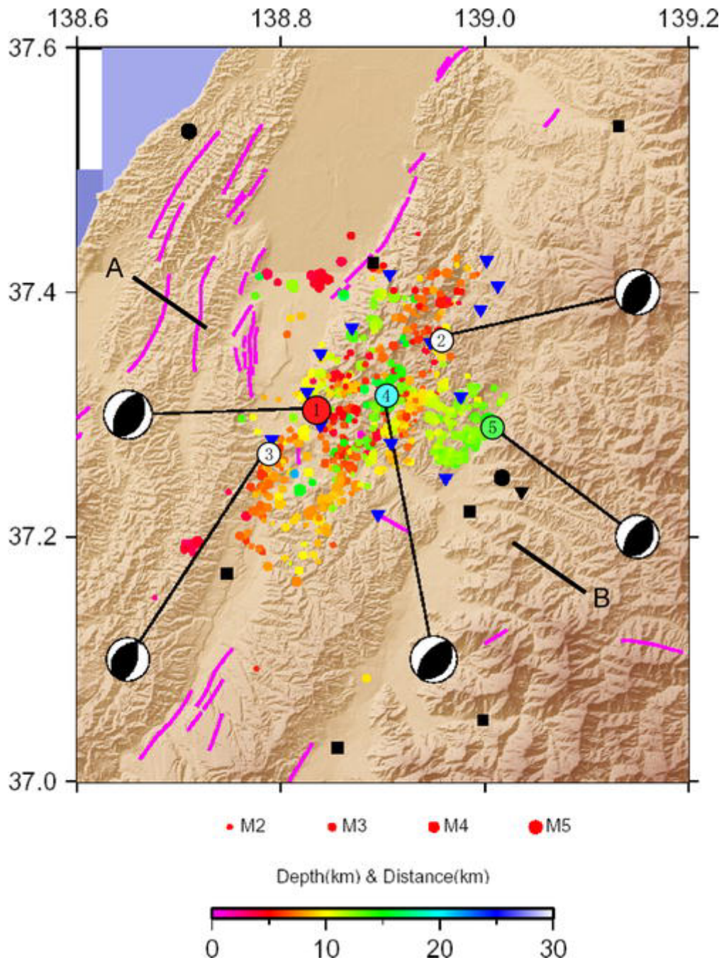
Fig. 3 Epicentral distribution determined from the present aftershock observation [18:00 JST Oct. 24 to 20:00 JST Oct. 27, 2004; data from Sakai et al. (2005)]. Aftershocks are denoted by color according to depth. There are 625 aftershocks plotted, among which the mainshock and large aftershocks are denoted by circles with numerals: 1. M6.8 mainshock (17:56 Oct. 23), 2. M6.3 aftershock (18:03 Oct. 23), 3. M6.0 aftershock (18:11 Oct. 23), 4. M6.5 aftershock (18:34 Oct. 23), 5. M6.1 aftershock (10:40 Oct. 27). Focal mechanisms are shown as projections on the lower focal hemisphere, where shaded areas indicate tension and white areas indicate compression. Active faults are denoted by solid pink lines
