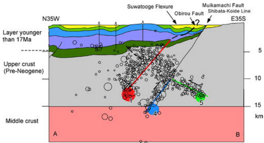
Fig. 4 Estimated geological cross-section showing the depth distribution of aftershocks determined from the present aftershock observation (see Fig. 3; after Hirata et al. 2005). 1. M6.8 mainshock (17:56 Oct. 23), 2. M6.3 aftershock (18:03 Oct. 23), 3. M6.0 aftershock (18:11 Oct. 23), 4. M6.5 aftershock (18:34 Oct. 23), 5. M6.1 aftershock (10:40 Oct. 27). Triangles denote location of wells of the Natural Gas Mining Society and the Society for Exploration for Oil on the Continental shelf (1992) and the Geological Information Center (1991). Colored solid lines indicate the three major source faults
