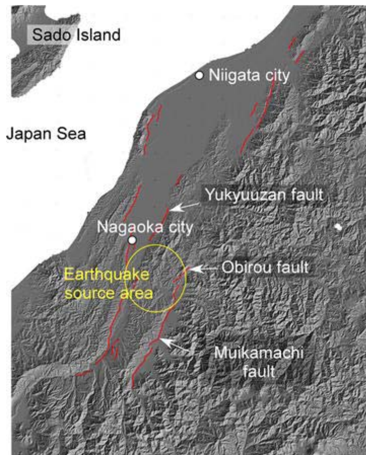
Fig. 2 Active faults near the source area of the 2004 Mid-Niigata Prefecture Earthquake. Red solid lines denote active faults (Geological Information Center 1991 ; Tsutsumi et al. 2001 ; Ikeda et al. 2002 ). The Muikamachi and Obirou faults are located on the eastern boundary of the Uonuma Hill
