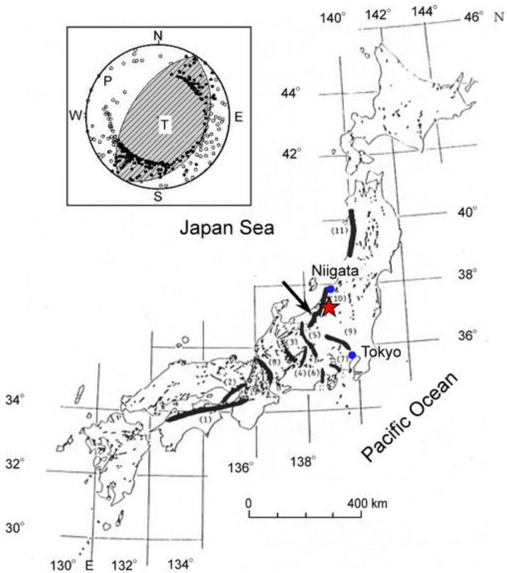
Fig. 1 Epicenter of the 2004 Mid-Niigata Prefecture Earthquake, with the focal mechanism shown inset as a stereo projection on the lower focal hemisphere, in which a shaded area indicates tension and white areas indicate compression. The mechanism shows a thrust faulting. Solid lines denote the 11 noteworthy active faults in Japan (Matsuda 1995 ), among which the western Nagaoka-plane fault system (indicated by an arrow) is the nearest active fault
