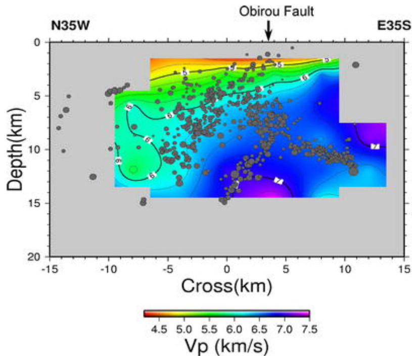
Fig. 5 P -wave velocity model (contour interval: 0.25 km/s) on the cross-section along the line A–B in Fig. 3 (after Kato et al. 2005) derived from data recorded by the 14 temporary stations of the present aftershock observation and 43 permanent stations
