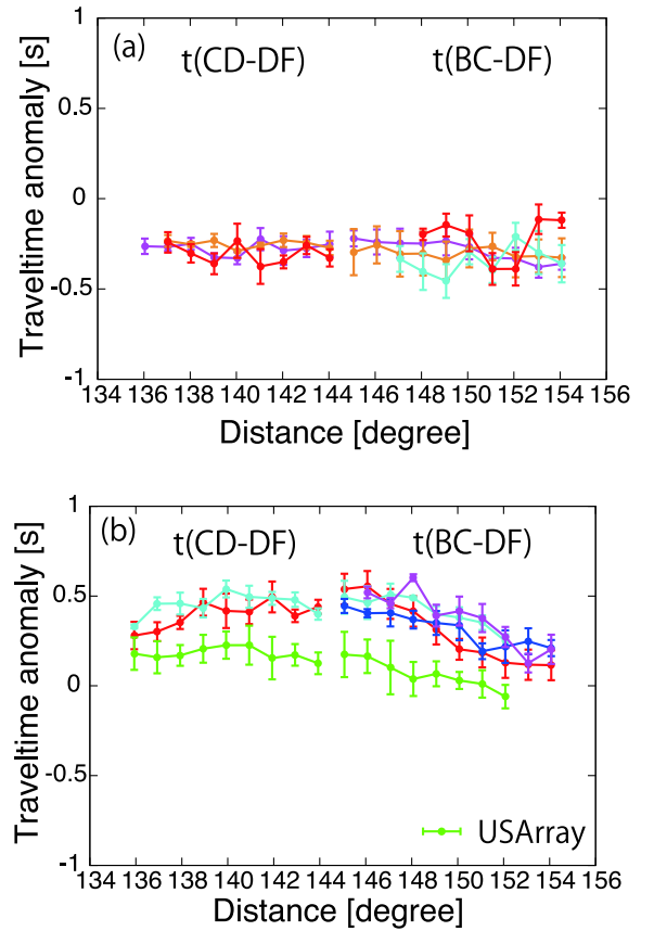
Fig. 10. Measured differential traveltime residuals referenced to AK135. Averaged values for each array for a distance bin of 1° are plotted; the distance range of 136–144° and 145–155° correspond the differential traveltime of PKP(DF)–PKP(CD) and PKP(DF)–PKP(BC), respectively. The error bar denotes the standard error and colors in (a) and (b) correspond to ray paths in Fig. 5a and c. (For interpretation of the references to color in this figure legend, the reader is referred to the web version of this article.)
