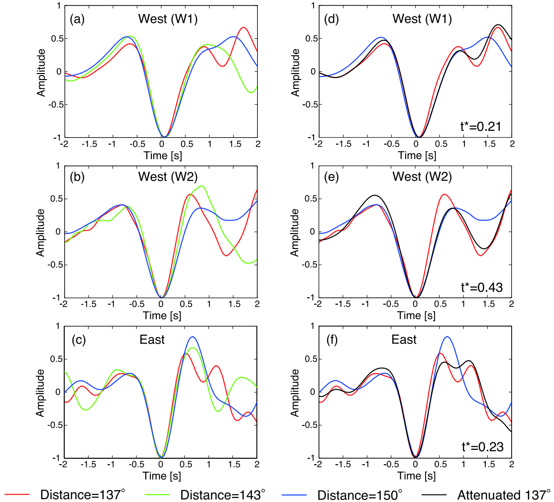
Fig. 6. (a–c) Comparison of stacked PKP(DF) phases for distance bins of 1^\circ around 137^\circ (red), 143^\circ (green) and 150^\circ (blue) for (a) W1 (event 19 July 2008 in Table 1), (b) W2 (8 June 2011) and (c) the eastern hemisphere (26 July 2005). (d–f) Similar to (a–c), but the observed waveform at 150^\circ (blue) is compared with the waveform of 137^\circ convolved with the attenuation filter with a differential value indicated at the right-bottom corner of each box (black). Waveforms are normalized by the maximum amplitudes. (For interpretation of the references to color in this figure legend, the reader is referred to the web version of this article.)
