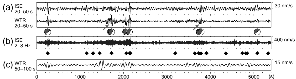
Figure 2. Observed vertical velocity waveforms during 90 minutes from 11 November 2008, 6:59 (GMT) at a N2-Array station ISE and a F-net station WTR (Figure 3(a)). (a) VLF waveforms and determined moment tensor solutions in lower-hemisphere projection. Arrows mark continuous signals of 100-300 s. (b) Tremor waveform and peak times used as the reference time for stacking (diamonds). (c) VLF waveform with a period longer than 50 s. Individual waveforms of other stations are too noisy to detect VLF signals in this frequency band.
