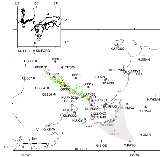
Fig. 1. Location map of the seismic stations. Crosses, small stars, triangles and circles indicate the permanent online, temporary online, temporary offline and temporary OBS stations, respectively. The epicenter distribution before the urgent joint observation period is also shown in the map. The large star represents the epicenter of the mainshock ( M_{JMA} 7.0 ), and the green dots denote the epicenters of aftershocks. The grey shaded area shows the Fukuoka metropolitan area.
