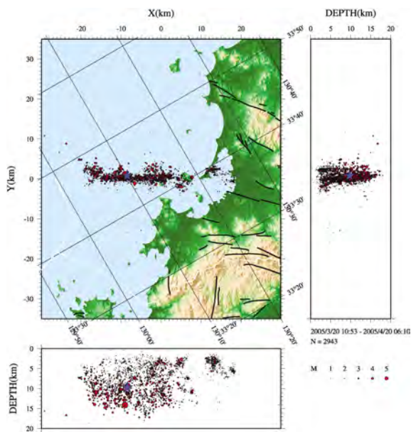
Fig. 2. Hypocenter distribution of the aftershocks before the largest aftershock of MJMA5.8 occurred (March 20–April 20, 2005). The star indicates the mainshock ( M_{JMA}7.0 ) on March 20. The distribution of active faults, as determined by the Research Group for Active Faults of Japan (1991), is shown by the thick lines in the map. Note that the map is rotated counterclockwise by 30^\circ so that the cross sections become approximately parallel and perpendicular to the alignment of aftershock distribution.
