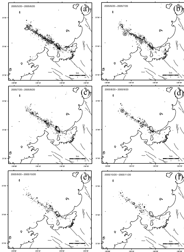
Fig. 4. Epicenter distributions of aftershocks from May 20 to November 20, 2005. The thick lines represent the active faults. The major aftershocks ( M > 4 ) are shown by the large circles. (a) May 20–June 20, 2005; (b) June 20–July 20, 2005; (c) July 20–August 20, 2005; (d) August 20–September 20, 2005; (e) September 20–October 20, 2005; (f) October 20–November 20, 2005.
