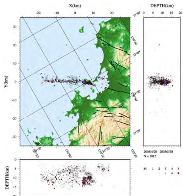
Fig. 3. Hypocenter distribution of the aftershocks during the month immediately following the largest aftershock (April 20–May 20, 2005). The star indicates the largest aftershock ( M_{JMA}5.8 ) on April 20. The cluster of the secondary aftershocks of the largest aftershock is recognized at the SE side of the largest aftershock.
