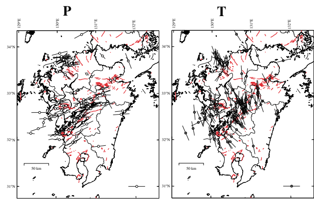
Fig. 5. Distribution of the principal stress orientation inferred from the focal mechanism solutions for the earthquakes shallower than 30 km in Kyushu. The results of the focal mechanism analysis for the 2005 West Off Fukuoka Prefecture Earthquake and its major aftershocks are included in the distribution of the principal stress orientation. (a) The maximum principal stresses (compression axes); (b) the minimum principal stresses (tension axes).
