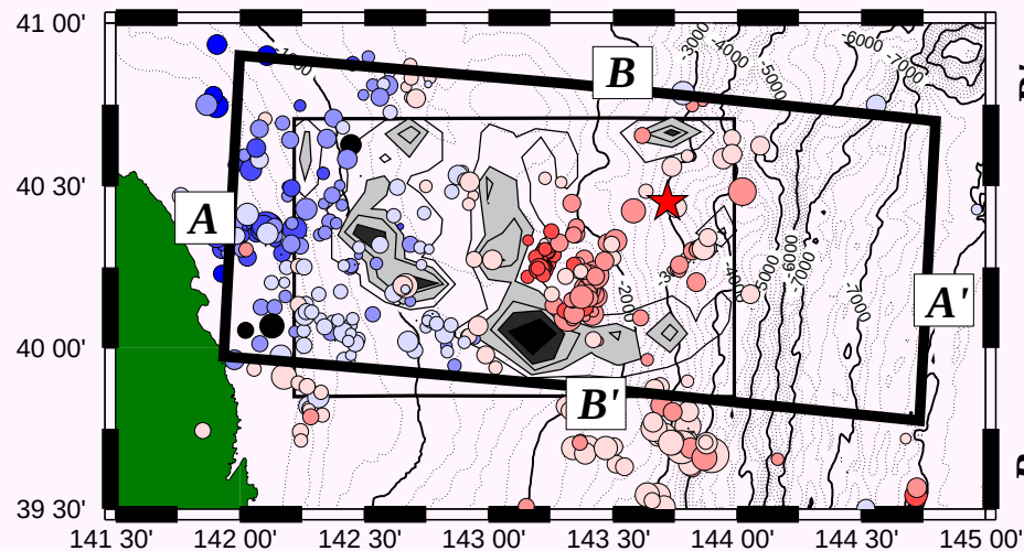
Aftershock Distribution (after Hino et al. , 2000)
