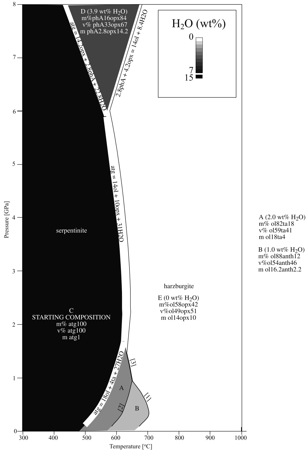
Figure 5. Phase diagram for serpentinite (see notes to Figure 2). [1] 2.2\text{fo} + 2.2\text{anth} = 9.9\text{en} + 2.2\text{H}_2\text{O} ; [2] 1.8\text{fo} + 4\text{ta} = 2.2\text{anth} + 1.8\text{H}_2\text{O} ; [3] 4\text{fo} + 4\text{ta} = 10\text{en} + 4\text{H}_2\text{O} .
